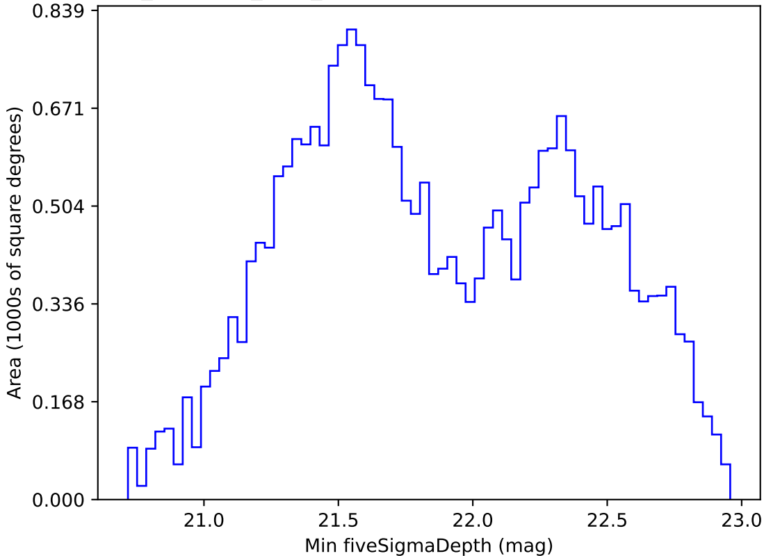
noroll_mjdp270_v3.4_10yrs All sky i band: Min fiveSigmaDepth
