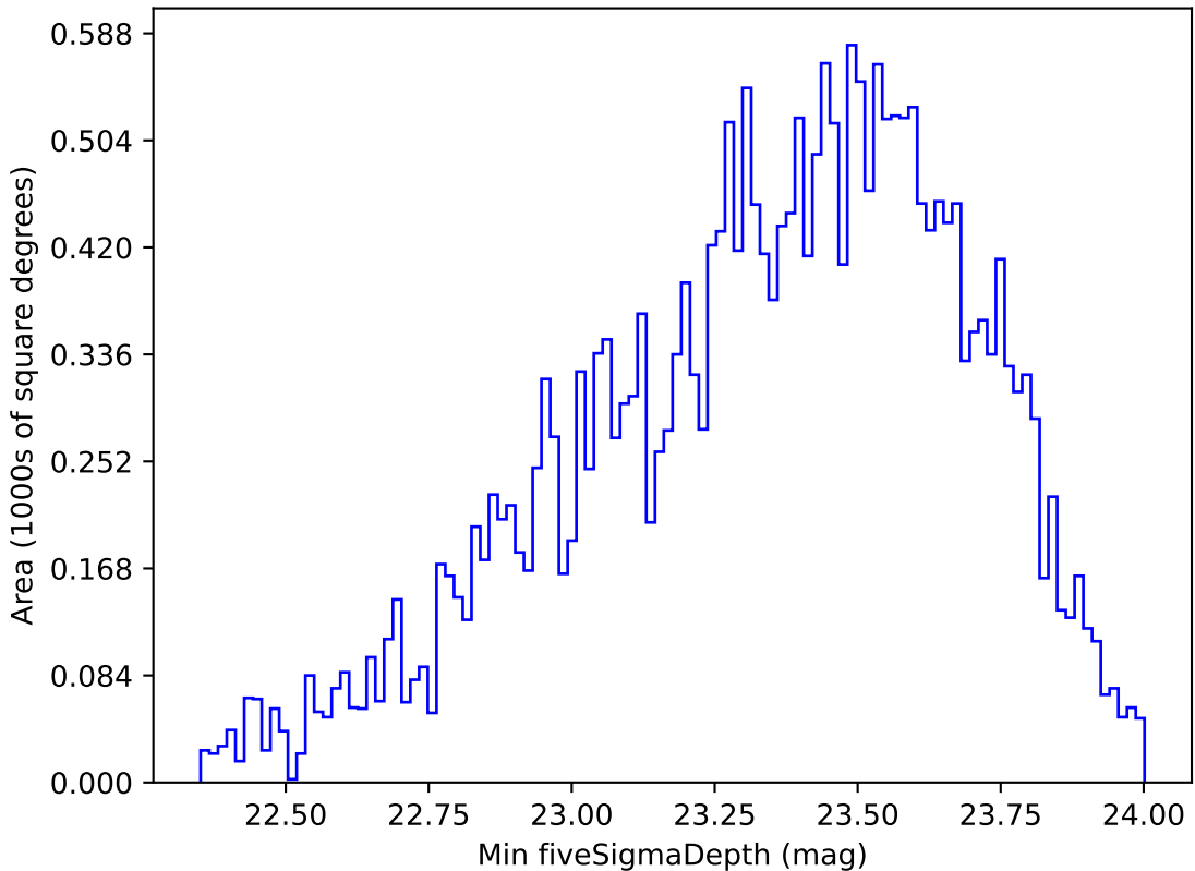
noroll_mjdp270_v3.4_10yrs All sky g band: Min fiveSigmaDepth
