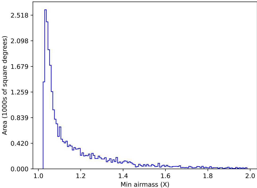
noroll_mjdp270_v3.4_10yrs Yr 1 z band: Min airmass
