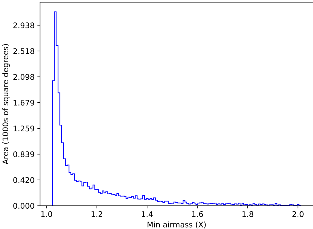
noroll_mjdp270_v3.4_10yrs Yr 1 r band: Min airmass
