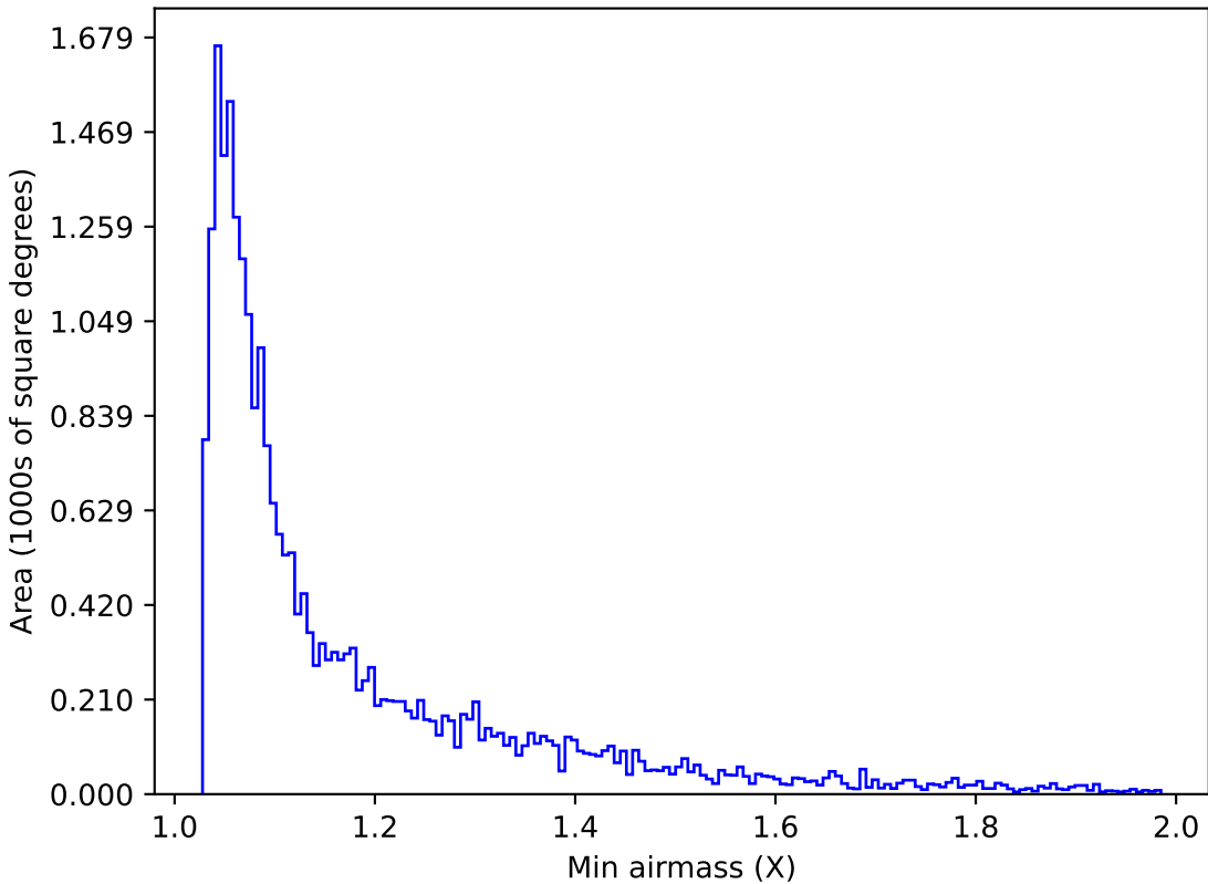
noroll_mjdp270_v3.4_10yrs Yr 1 g band: Min airmass
