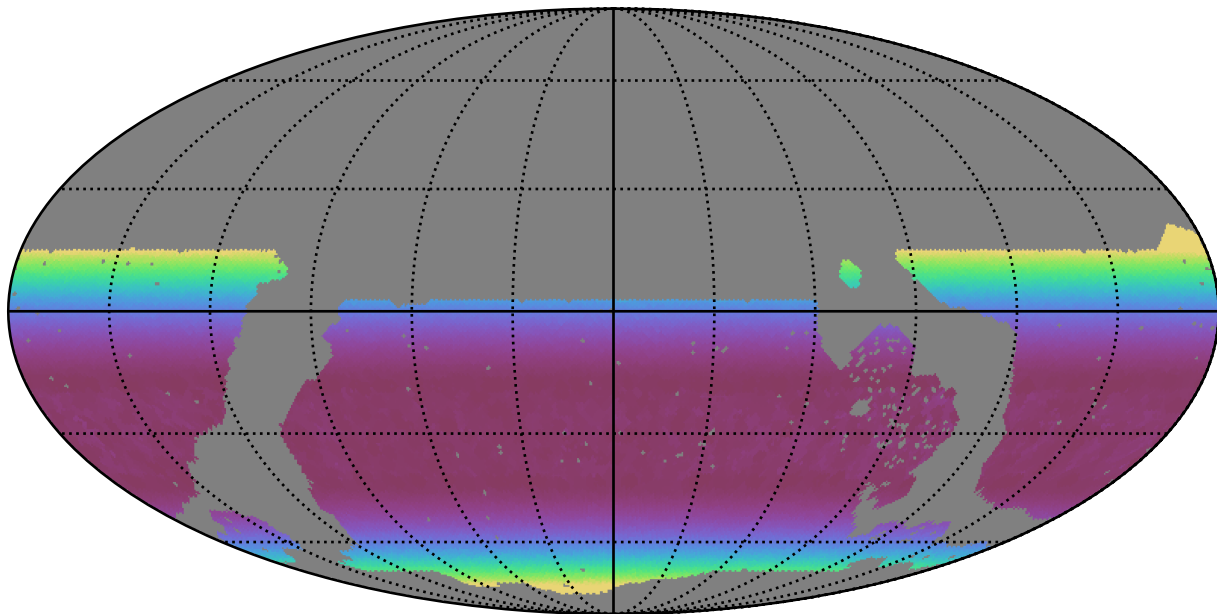
noroll_mjdp270_v3.4_10yrs WFD y band: Min airmass
