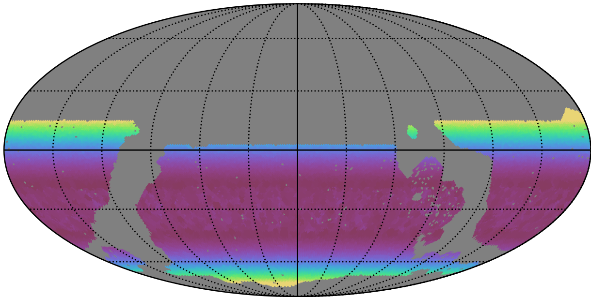
noroll_mjdp270_v3.4_10yrs WFD u band: Min airmass
