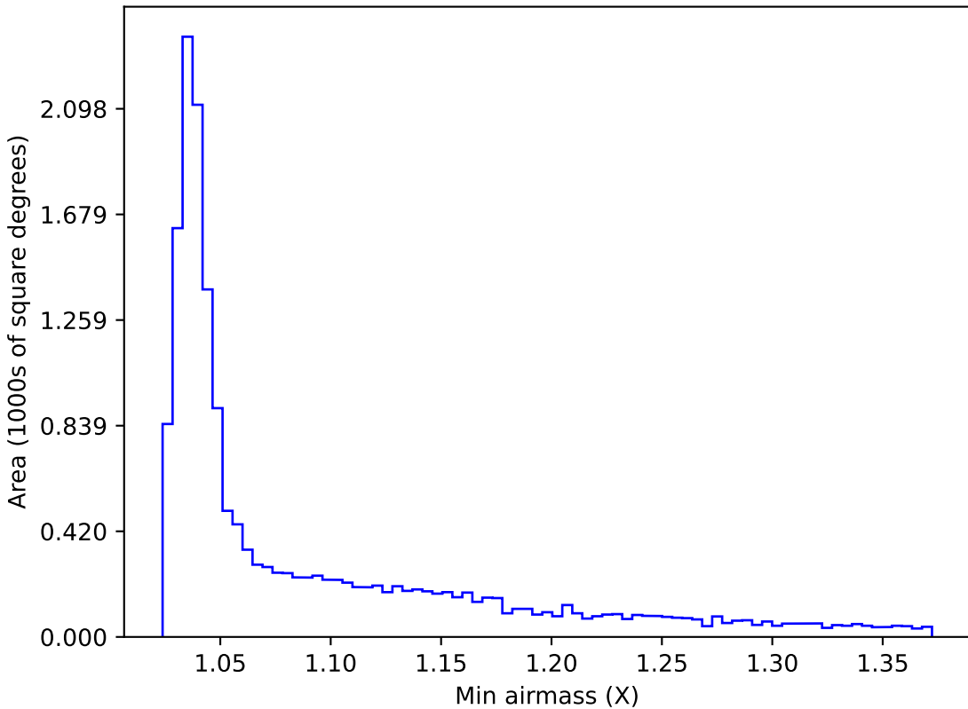
noroll_mjdp270_v3.4_10yrs WFD u band: Min airmass
