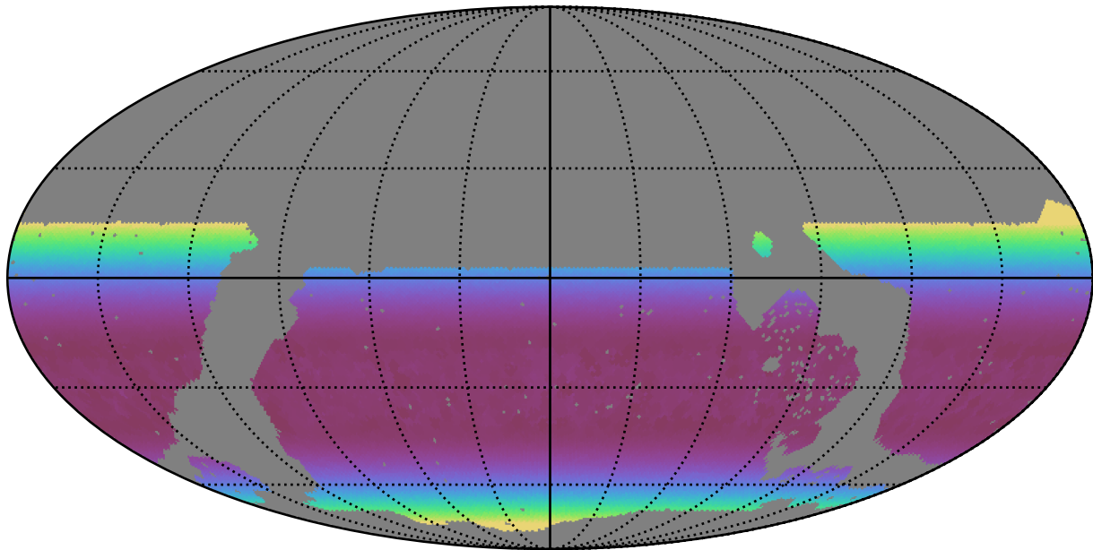
noroll_mjdp270_v3.4_10yrs WFD r band: Min airmass
