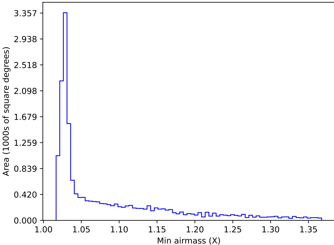
noroll_mjdp270_v3.4_10yrs WFD r band: Min airmass
