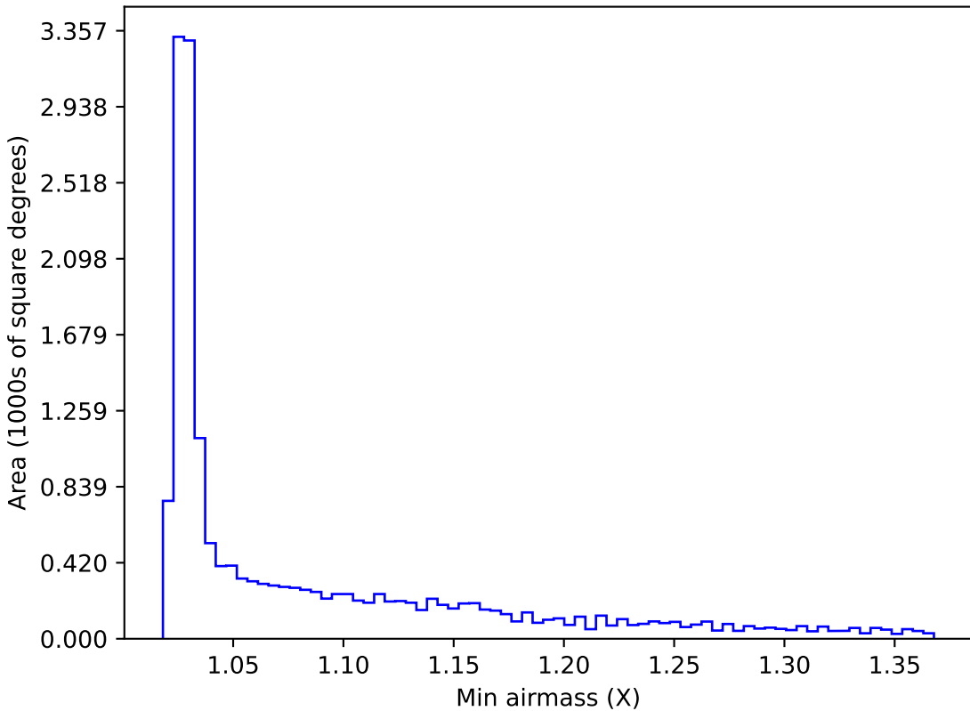
noroll_mjdp270_v3.4_10yrs WFD i band: Min airmass
