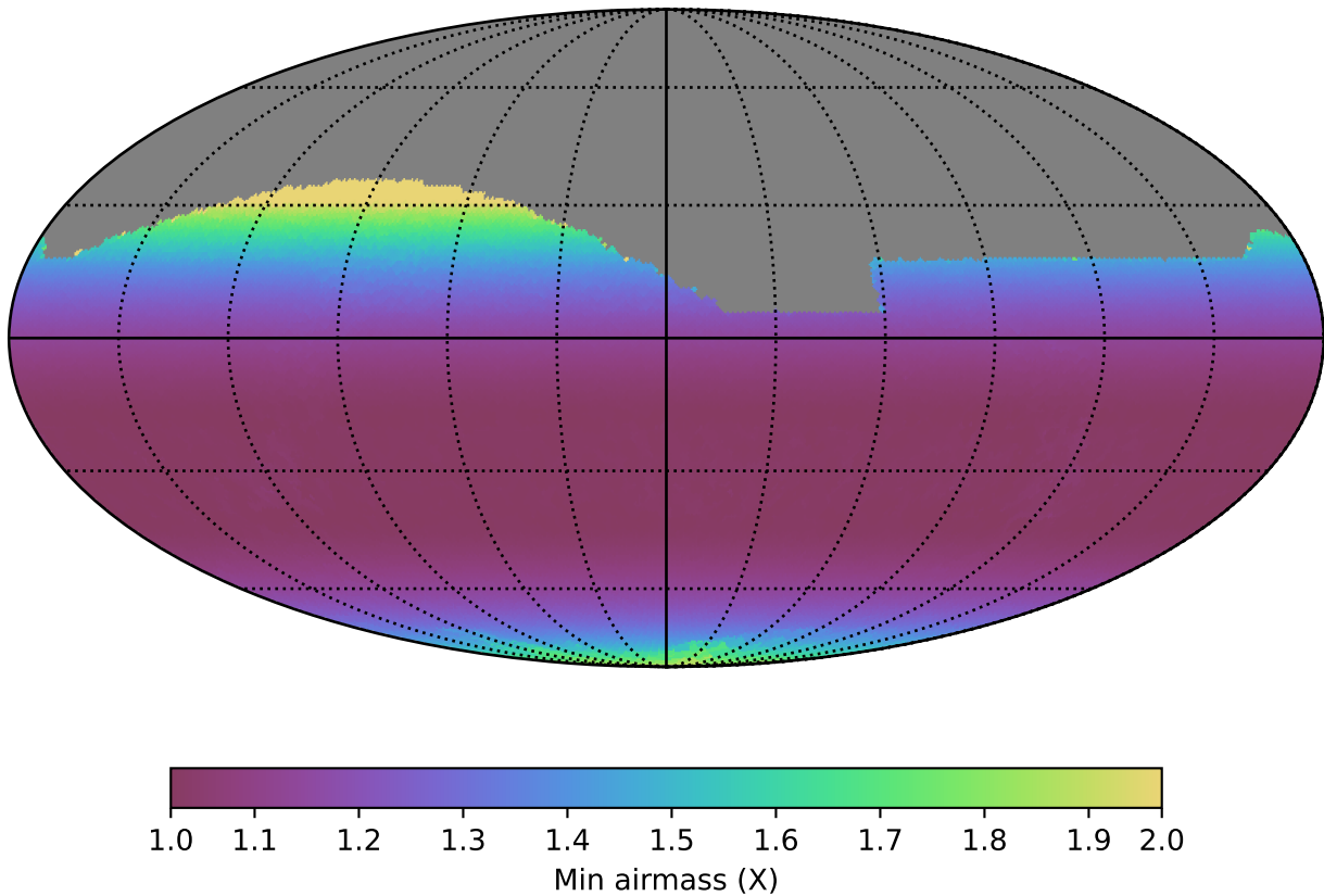
noroll_mjdp270_v3.4_10yrs All sky z band: Min airmass
