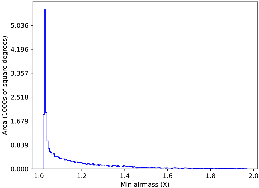
noroll_mjdp270_v3.4_10yrs All sky z band: Min airmass
