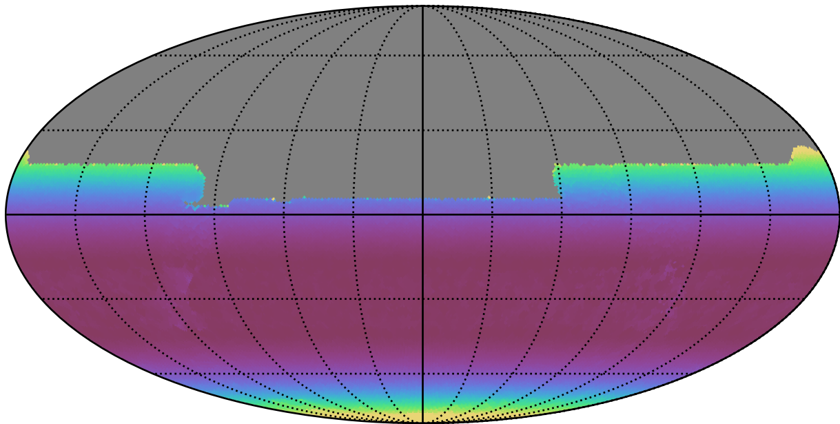
noroll_mjdp270_v3.4_10yrs All sky y band: Min airmass
