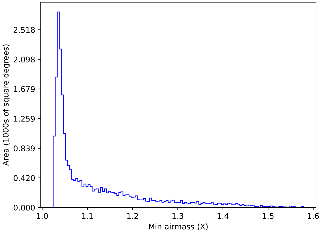
noroll_mjdp270_v3.4_10yrs All sky u band: Min airmass
