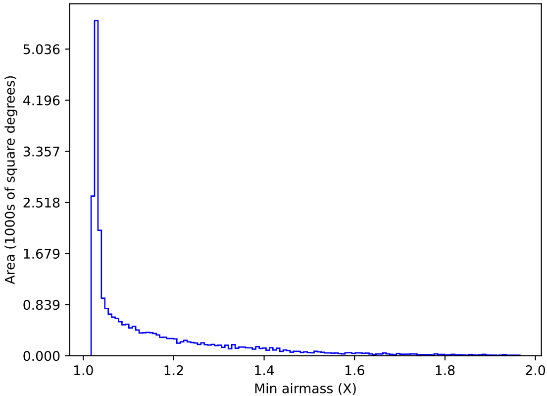
noroll_mjdp270_v3.4_10yrs All sky r band: Min airmass
