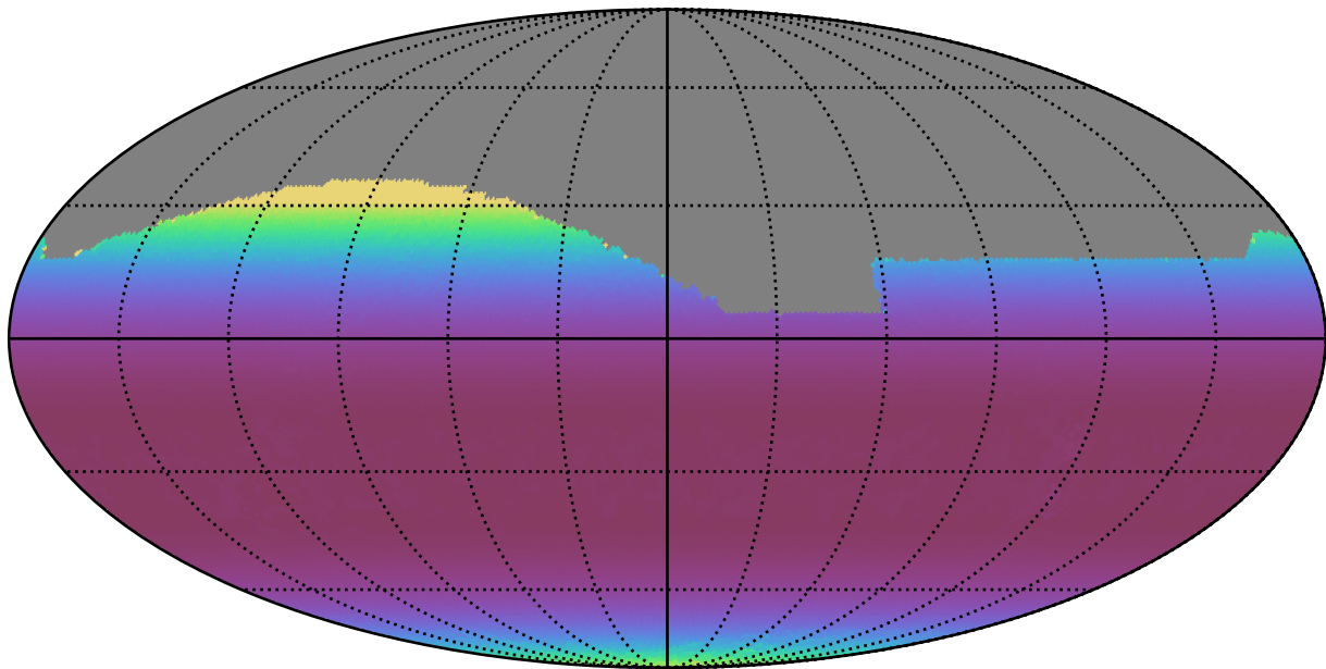
noroll_mjdp270_v3.4_10yrs All sky i band: Min airmass
