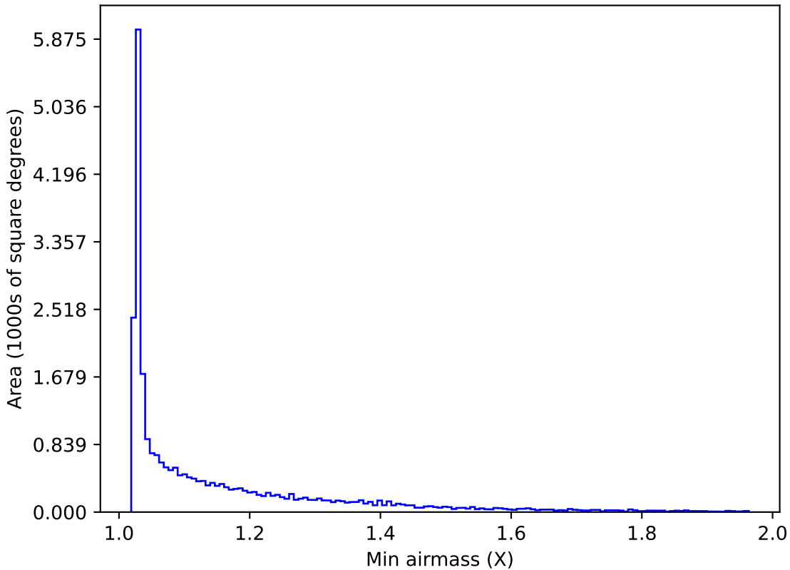
noroll_mjdp270_v3.4_10yrs All sky i band: Min airmass
