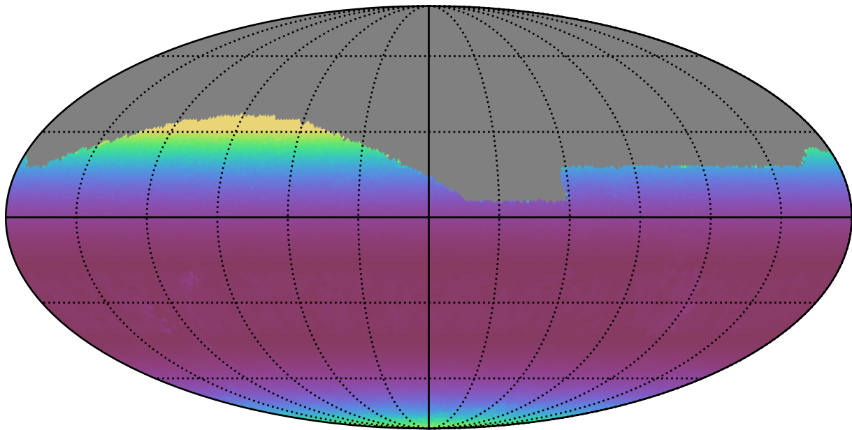
noroll_mjdp270_v3.4_10yrs All sky g band: Min airmass
