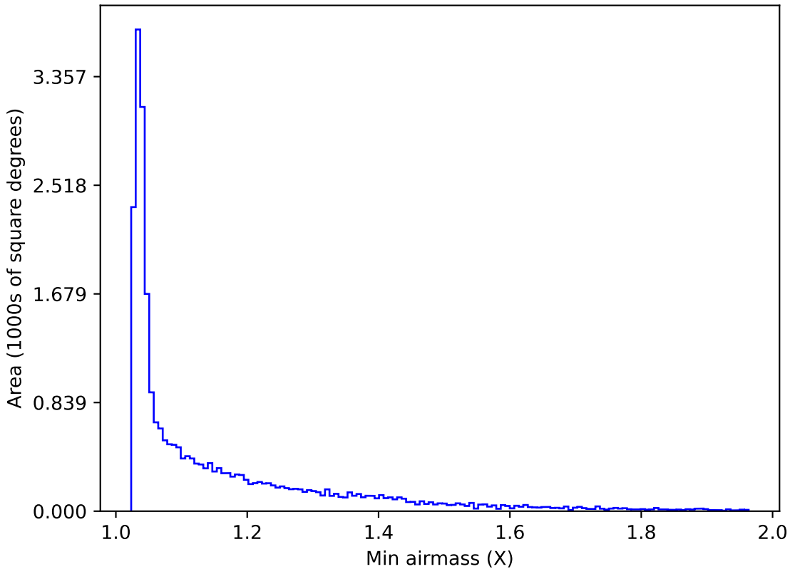
noroll_mjdp270_v3.4_10yrs All sky g band: Min airmass
