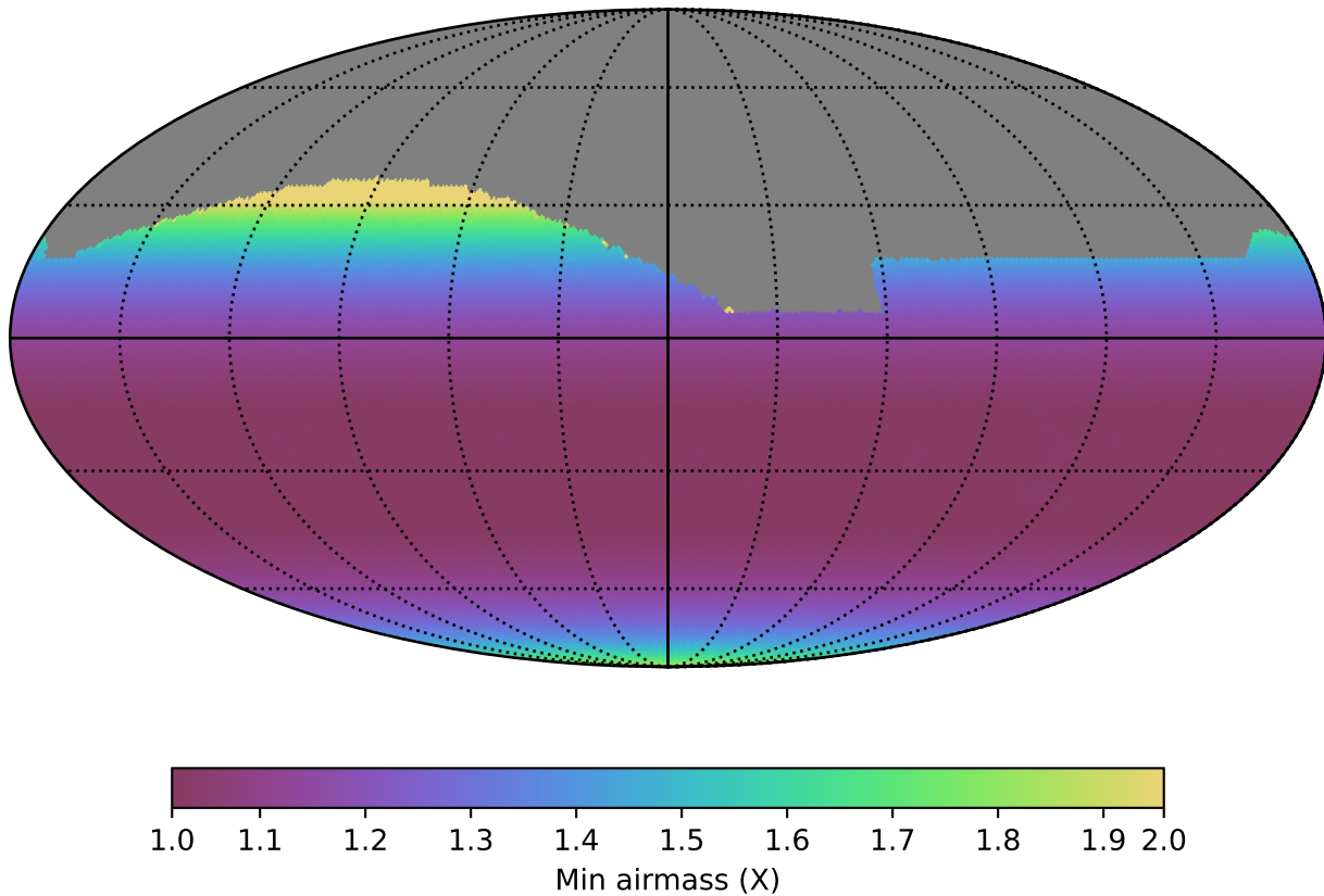
noroll_mjdp270_v3.4_10yrs All sky all bands: Min airmass
