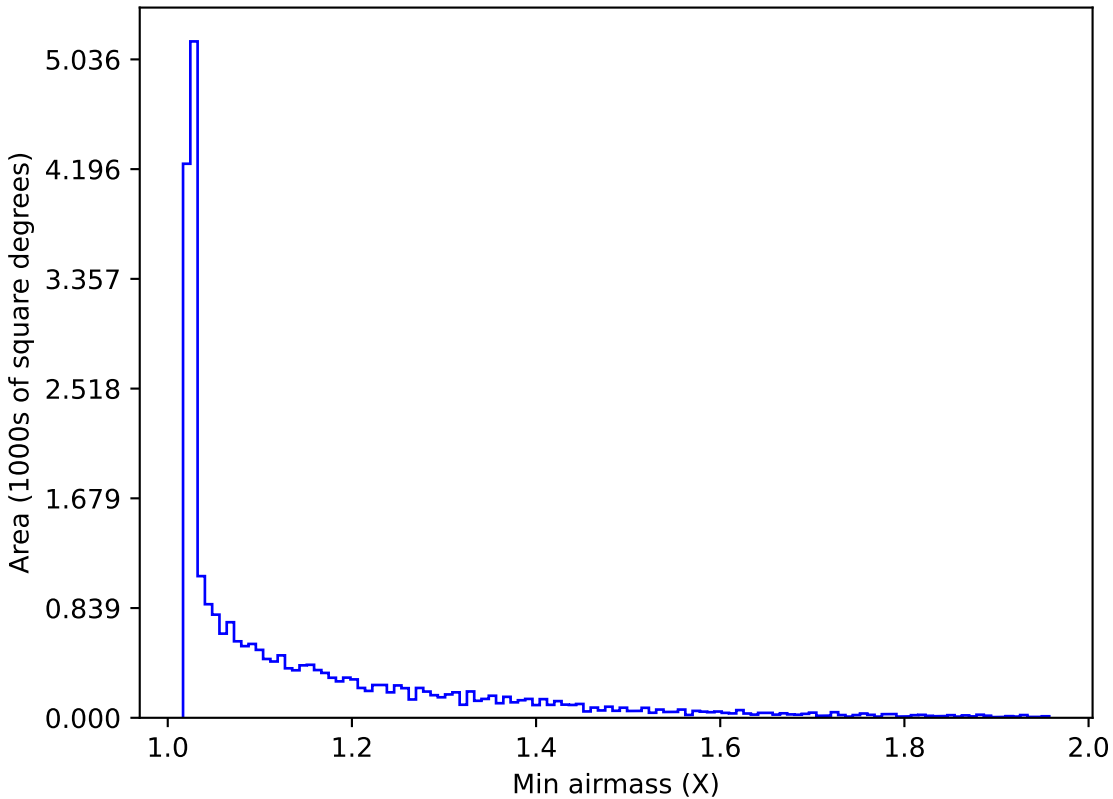
noroll_mjdp270_v3.4_10yrs All sky all bands: Min airmass
