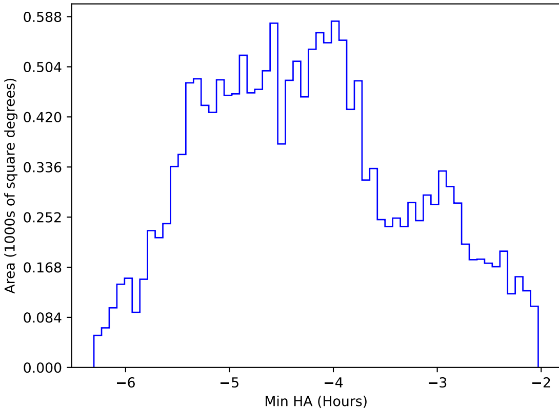
noroll_mjdp270_v3.4_10yrs WFD r band: Min HA
