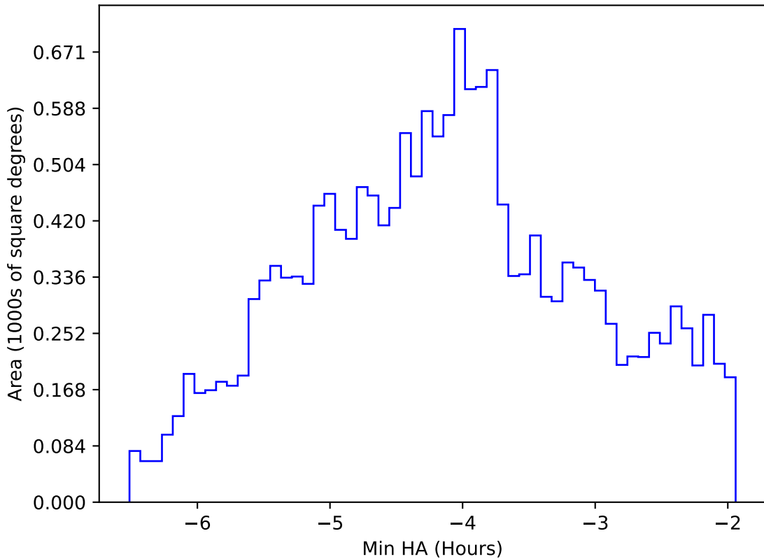
noroll_mjdp270_v3.4_10yrs WFD i band: Min HA
