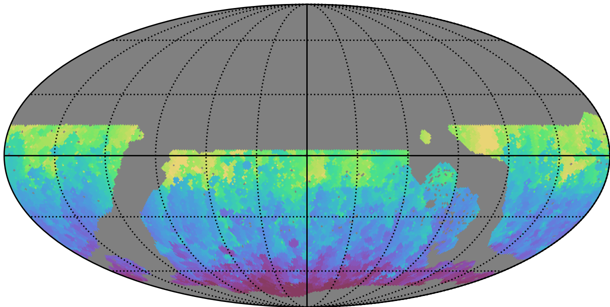
noroll_mjdp270_v3.4_10yrs WFD g band: Min HA
