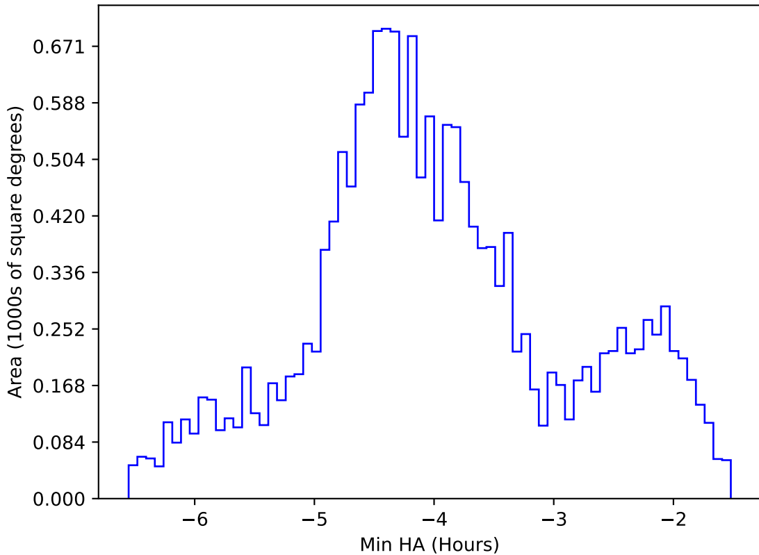
noroll_mjdp270_v3.4_10yrs WFD g band: Min HA
