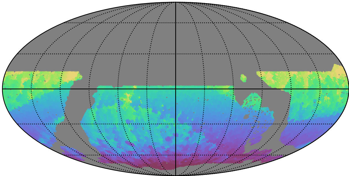
noroll_mjdp270_v3.4_10yrs WFD all bands: Min HA
