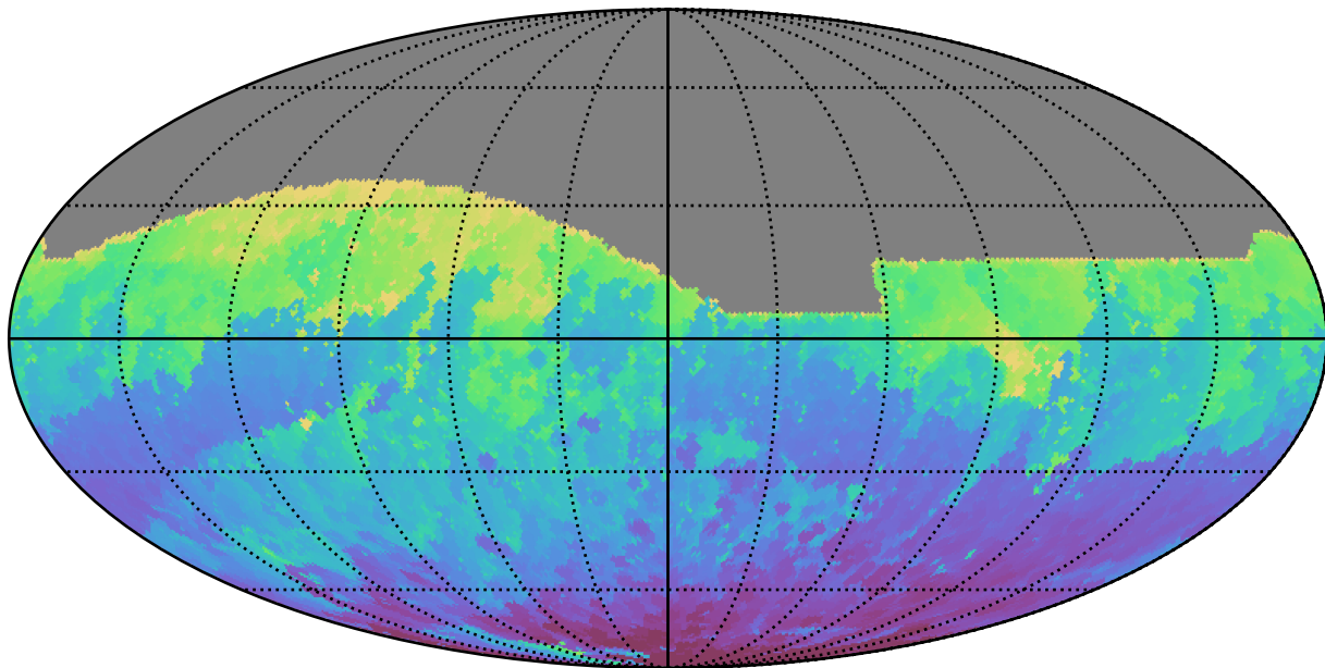
noroll_mjdp270_v3.4_10yrs All sky z band: Min HA
