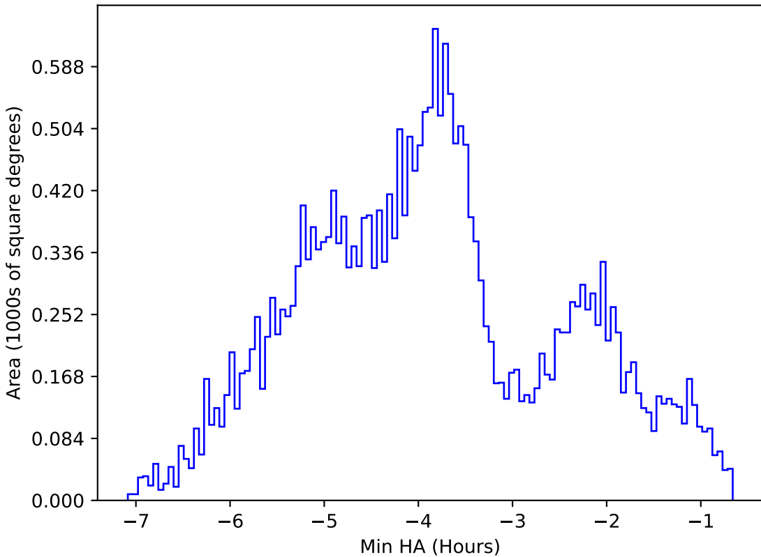
noroll_mjdp270_v3.4_10yrs All sky z band: Min HA
