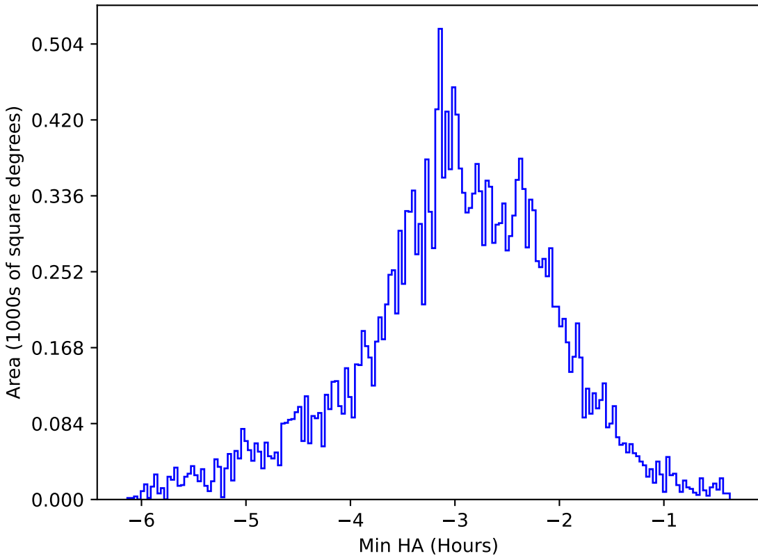
noroll_mjdp270_v3.4_10yrs All sky u band: Min HA
