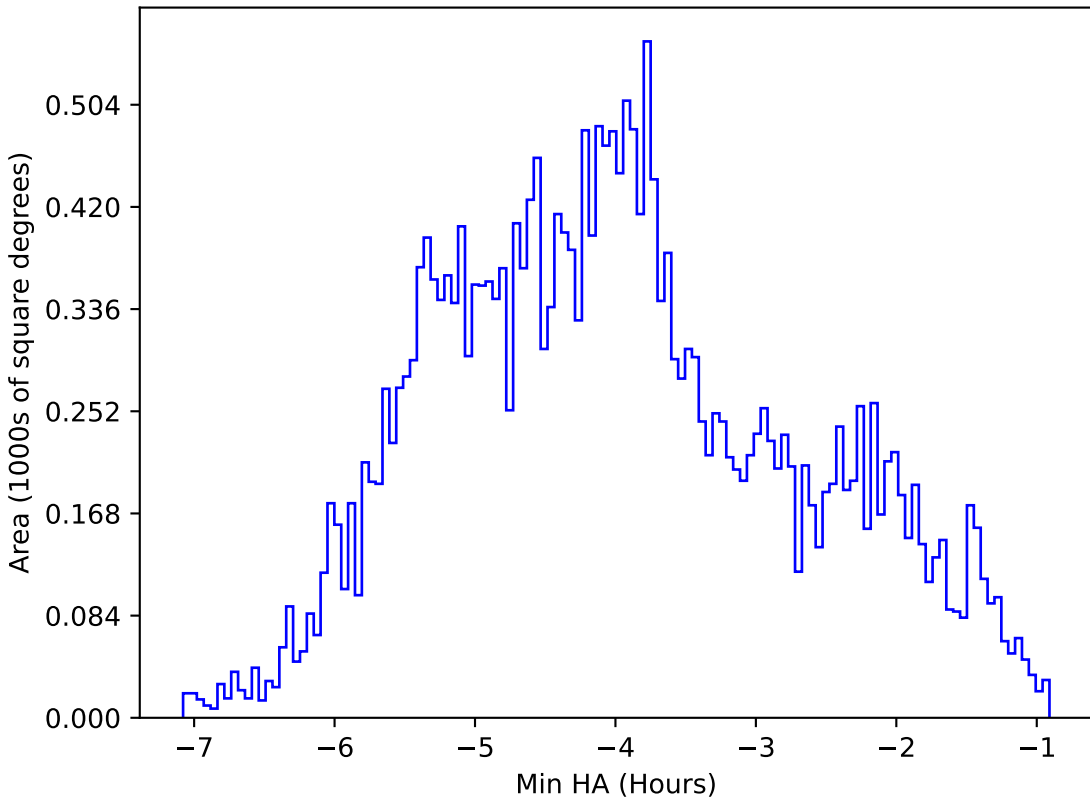
noroll_mjdp270_v3.4_10yrs All sky r band: Min HA
