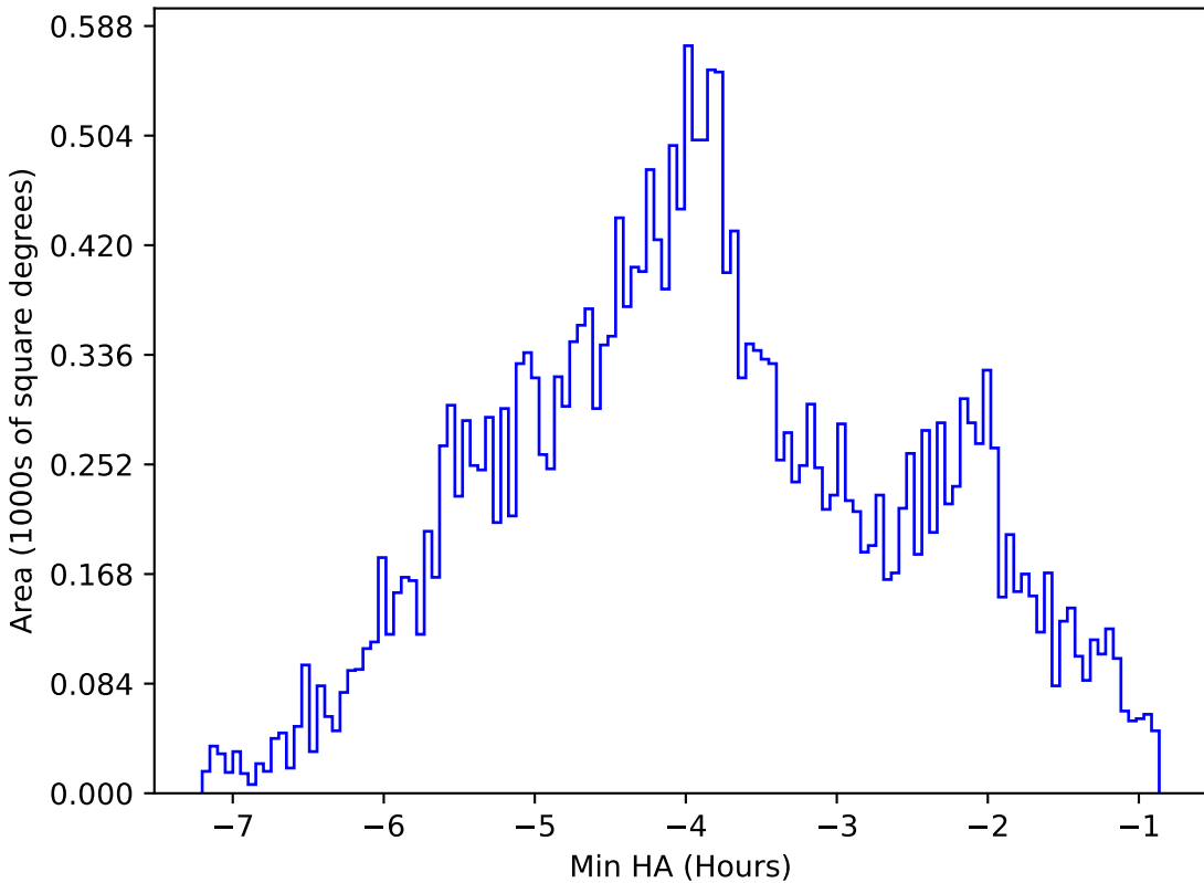
noroll_mjdp270_v3.4_10yrs All sky i band: Min HA
