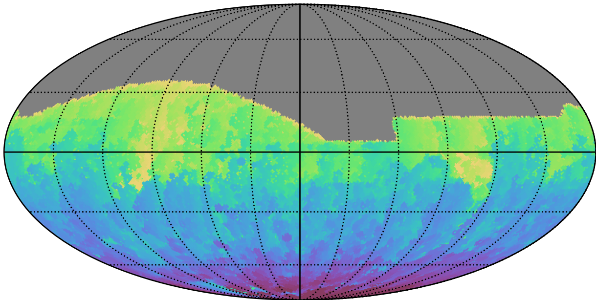
noroll_mjdp270_v3.4_10yrs All sky g band: Min HA
