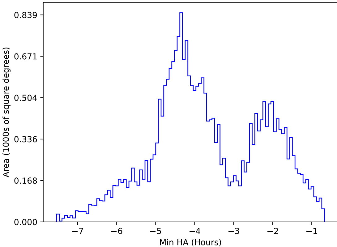
noroll_mjdp270_v3.4_10yrs All sky g band: Min HA
