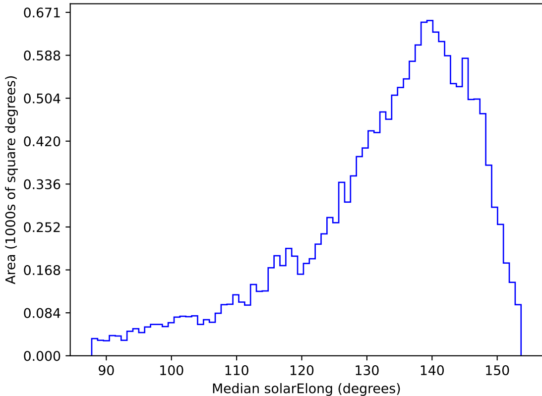
noroll_mjdp270_v3.4_10yrs WFD u band: Median solarElong
