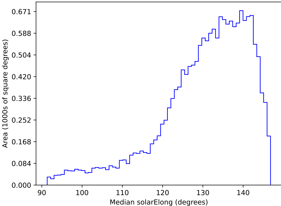
noroll_mjdp270_v3.4_10yrs WFD r band: Median solarElong
