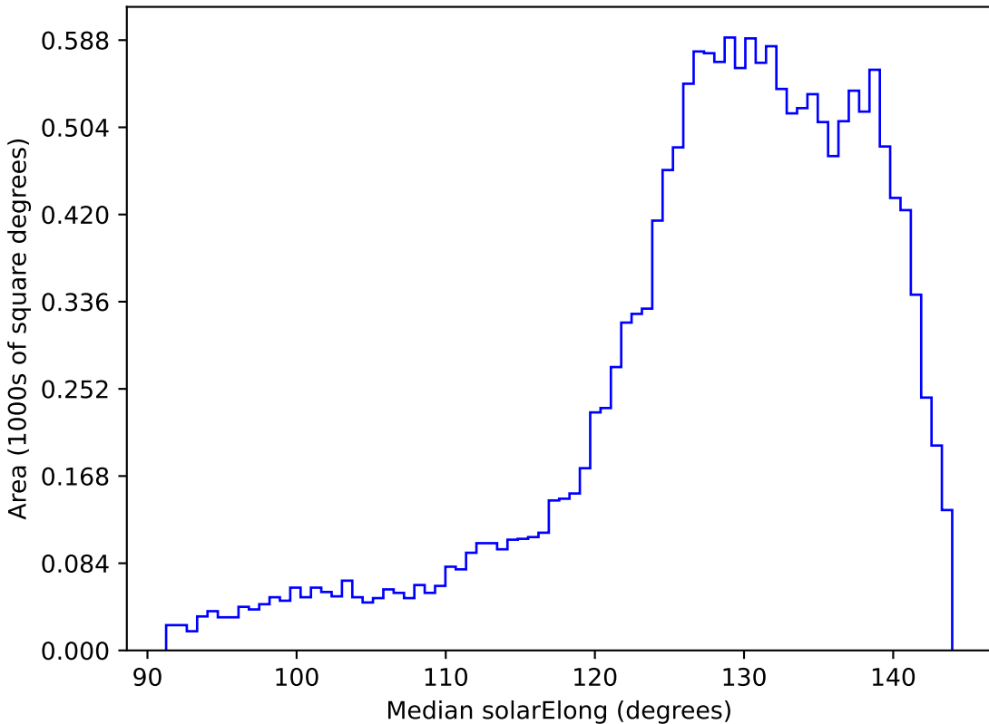
noroll_mjdp270_v3.4_10yrs WFD i band: Median solarElong
