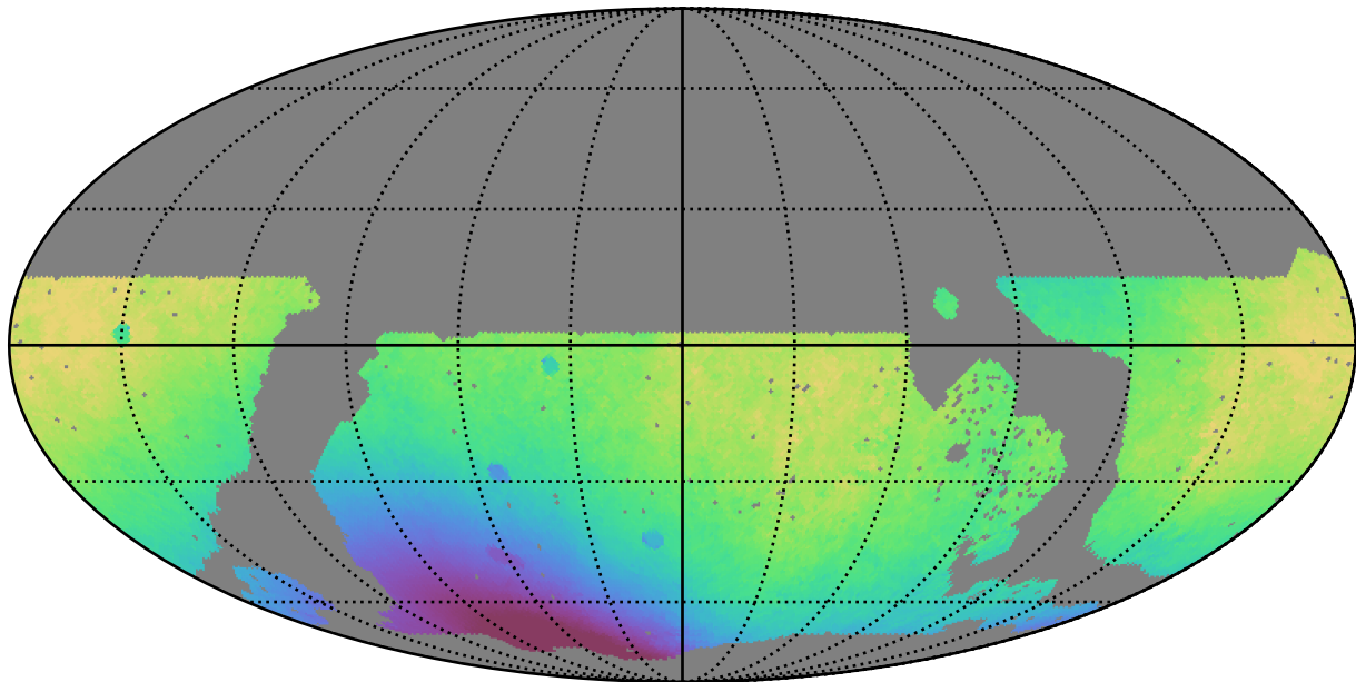
noroll_mjdp270_v3.4_10yrs WFD all bands: Median solarElong
