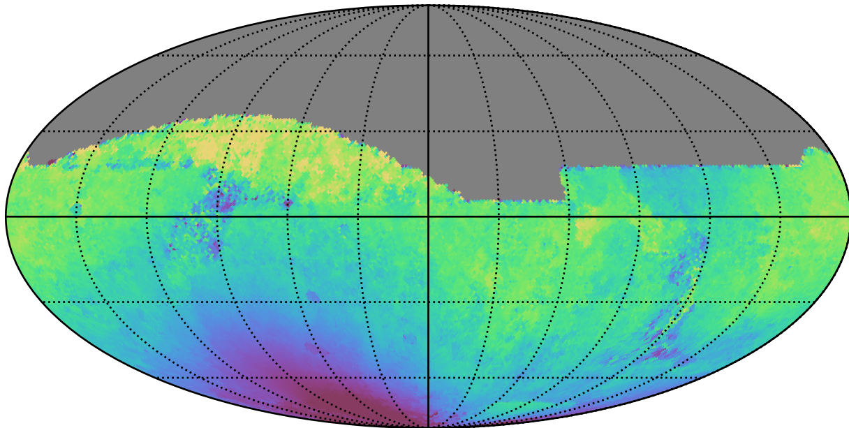
noroll_mjdp270_v3.4_10yrs All sky z band: Median solarElong
