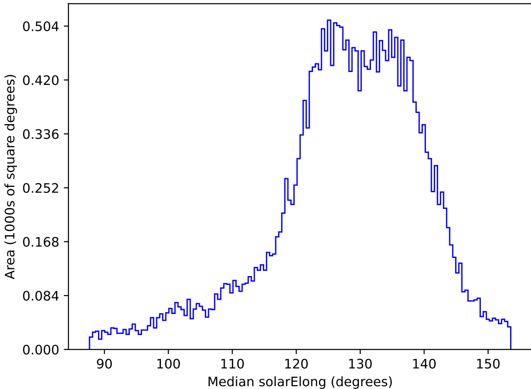
noroll_mjdp270_v3.4_10yrs All sky z band: Median solarElong
