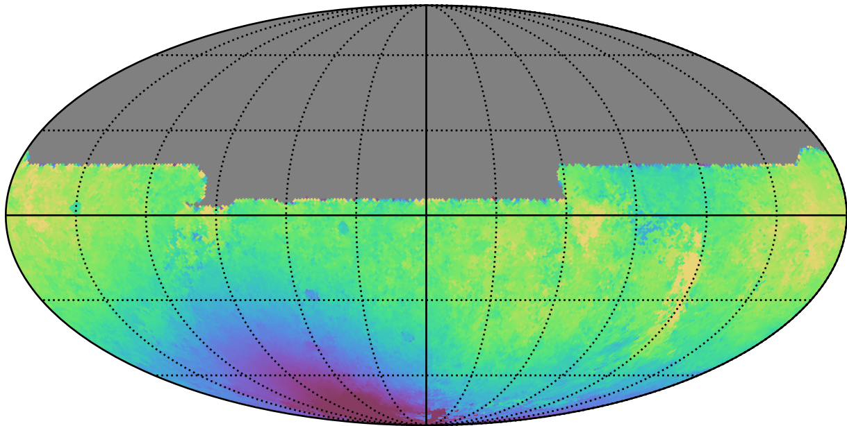
noroll_mjdp270_v3.4_10yrs All sky y band: Median solarElong
