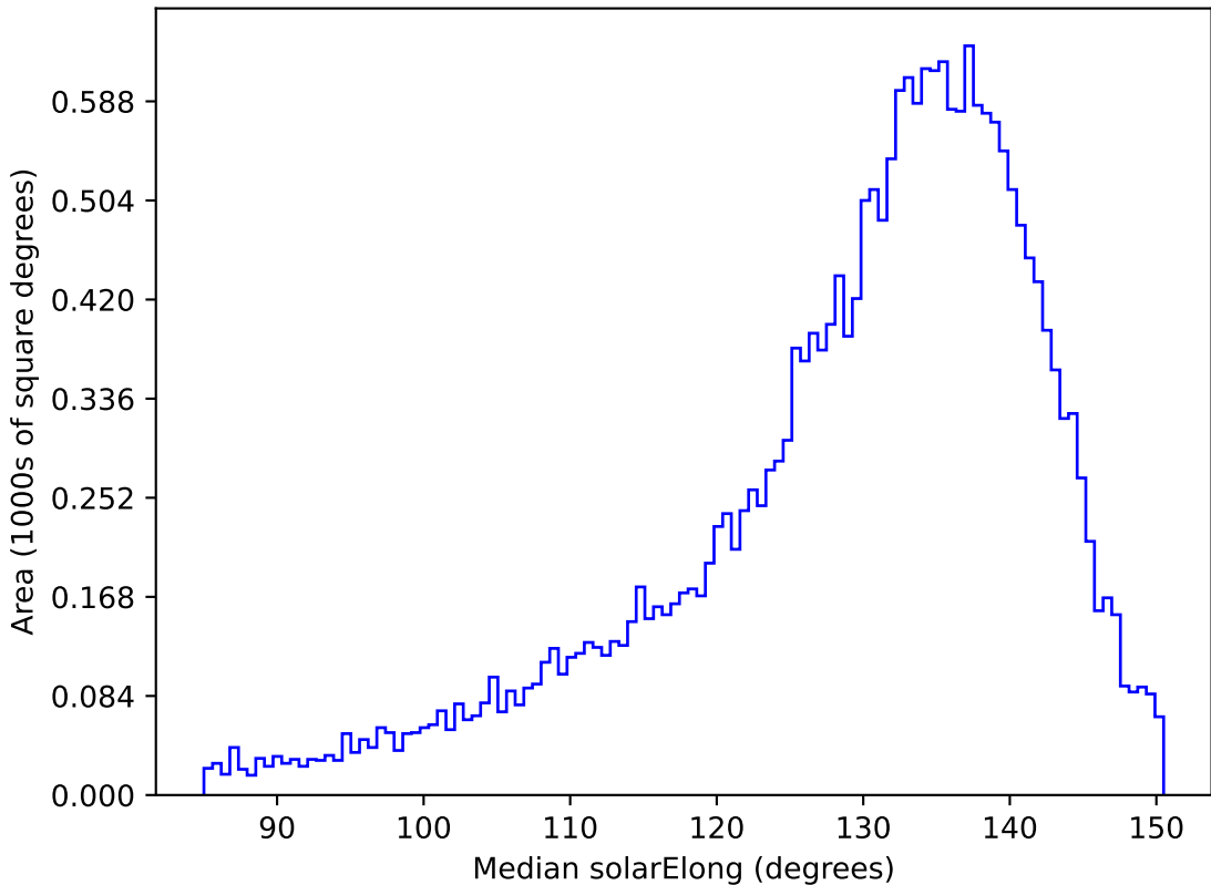
noroll_mjdp270_v3.4_10yrs All sky y band: Median solarElong
