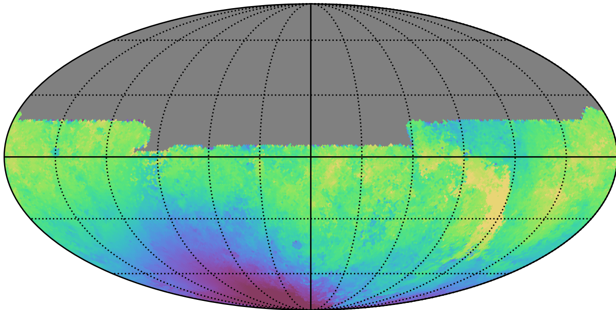
noroll_mjdp270_v3.4_10yrs All sky u band: Median solarElong
