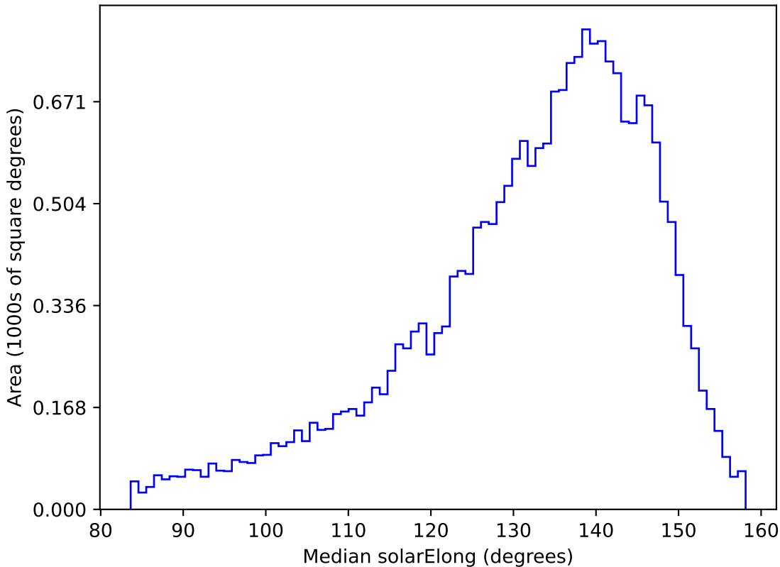
noroll_mjdp270_v3.4_10yrs All sky u band: Median solarElong
