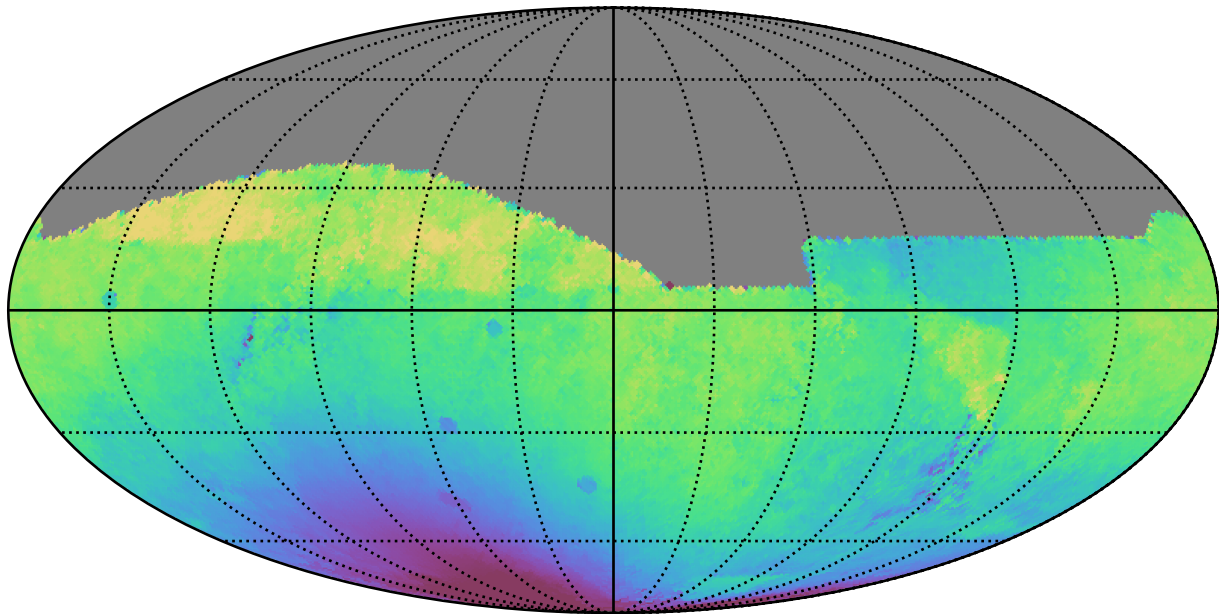
noroll_mjdp270_v3.4_10yrs All sky r band: Median solarElong
