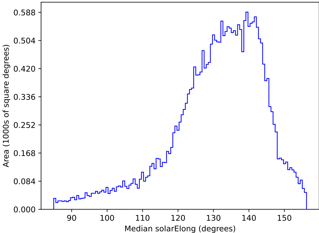
noroll_mjdp270_v3.4_10yrs All sky r band: Median solarElong
