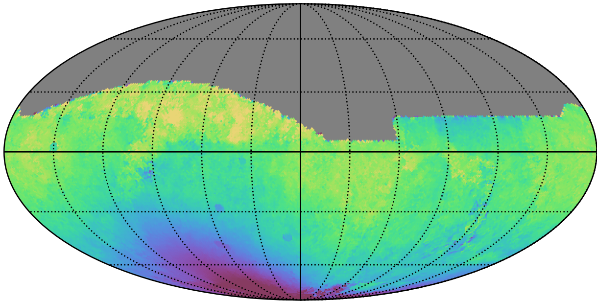
noroll_mjdp270_v3.4_10yrs All sky i band: Median solarElong
