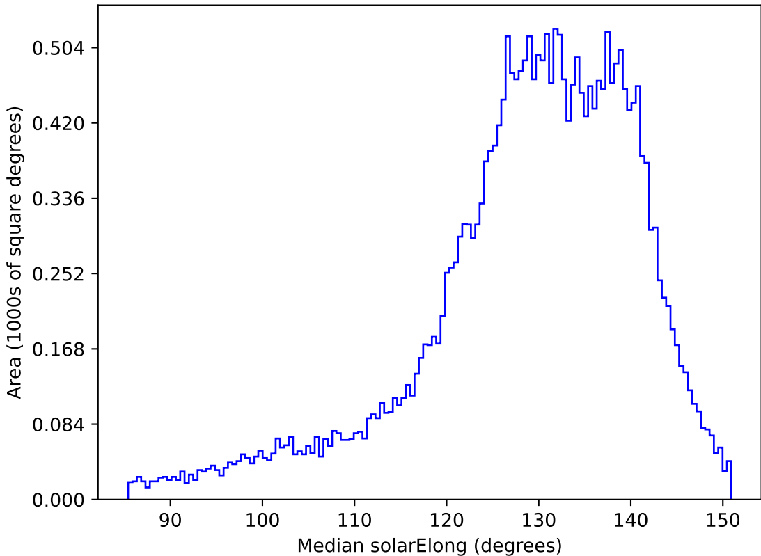
noroll_mjdp270_v3.4_10yrs All sky i band: Median solarElong
