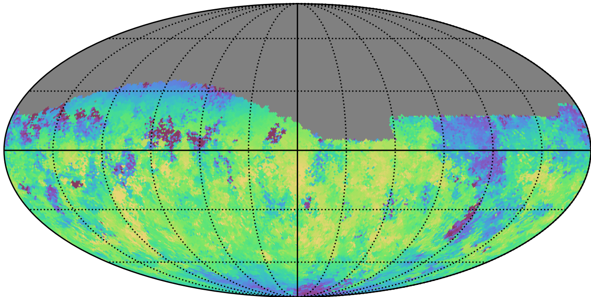
noroll_mjdp270_v3.4_10yrs Yr 1 z band: Median skyBrightness
