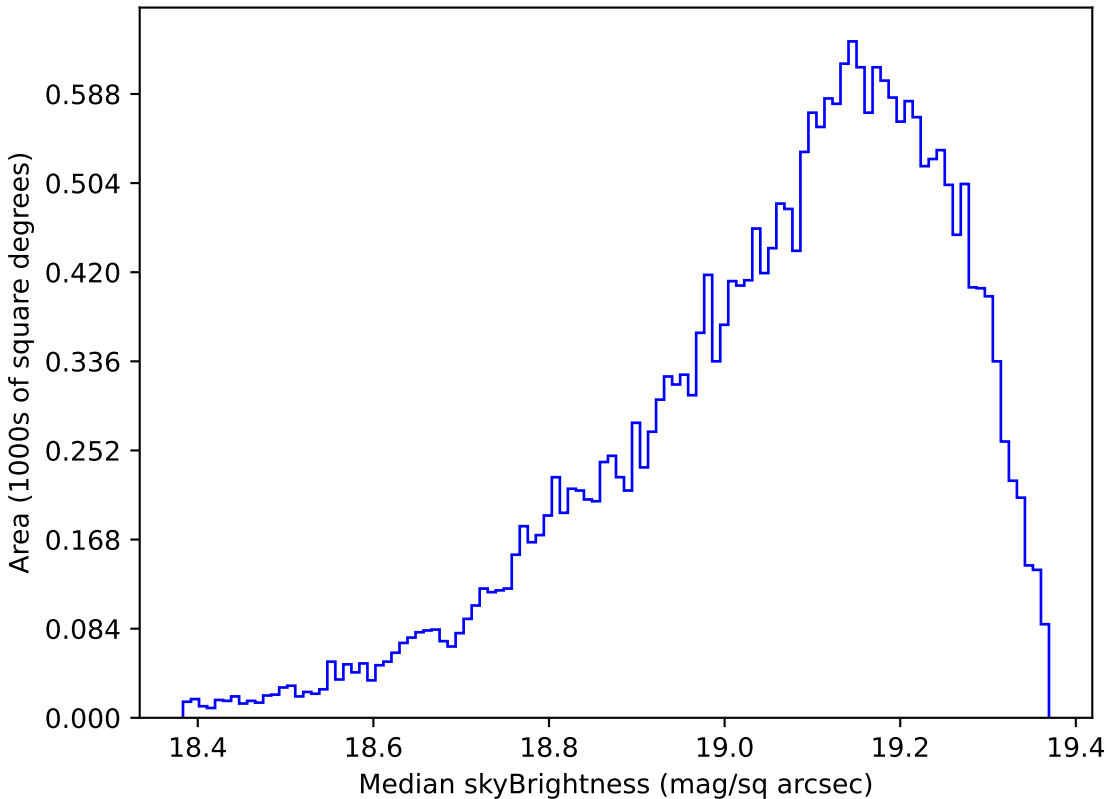
noroll_mjdp270_v3.4_10yrs Yr 1 z band: Median skyBrightness
